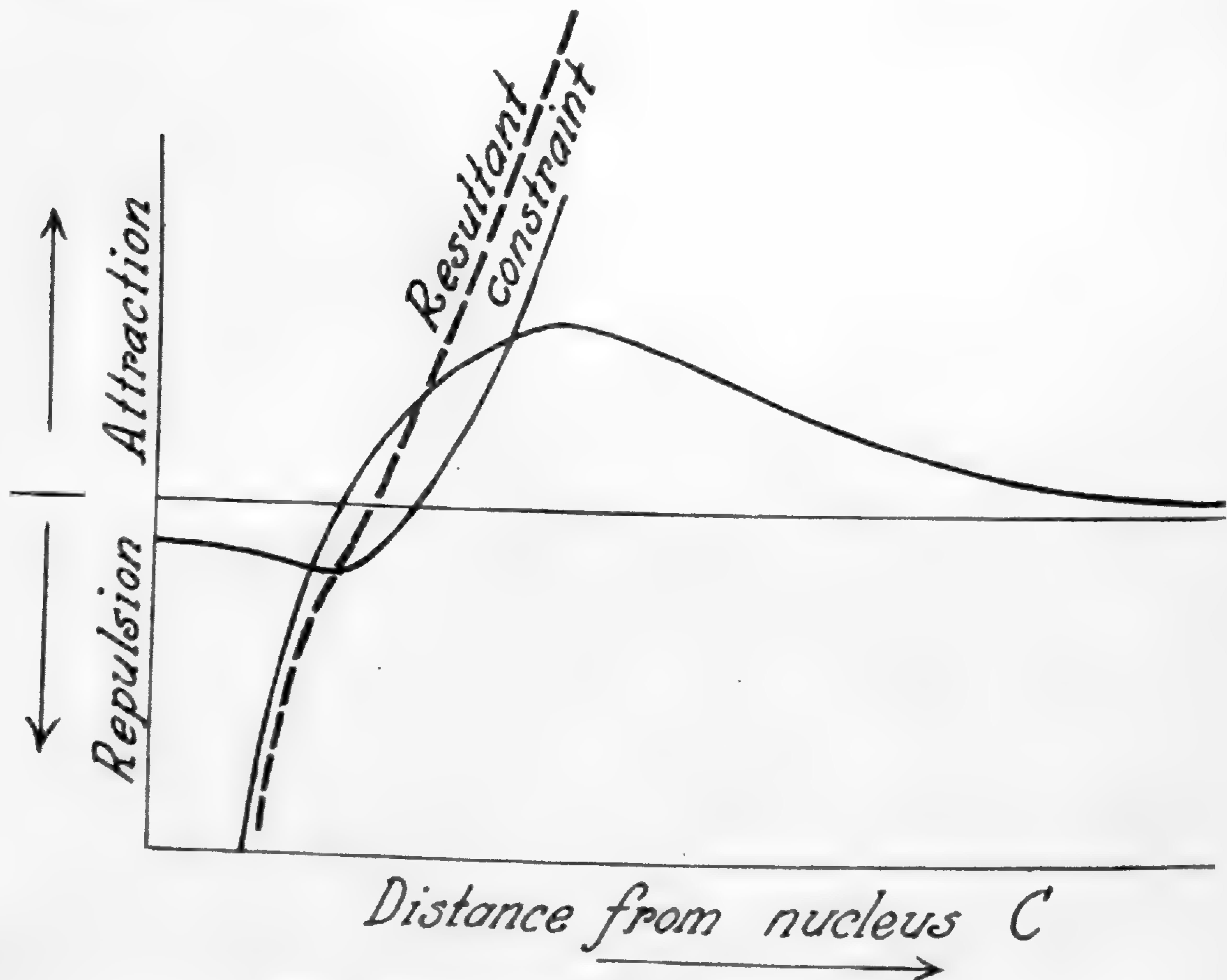
FIG. 4. Unsymmetrical weak union; firm electron.
